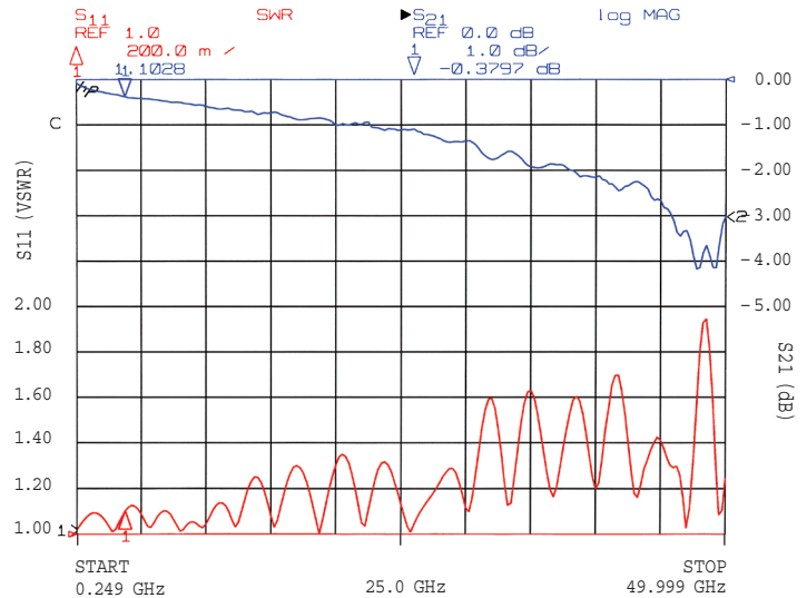
Test data original 30 mil coplanar test board (Serial Number 0).
