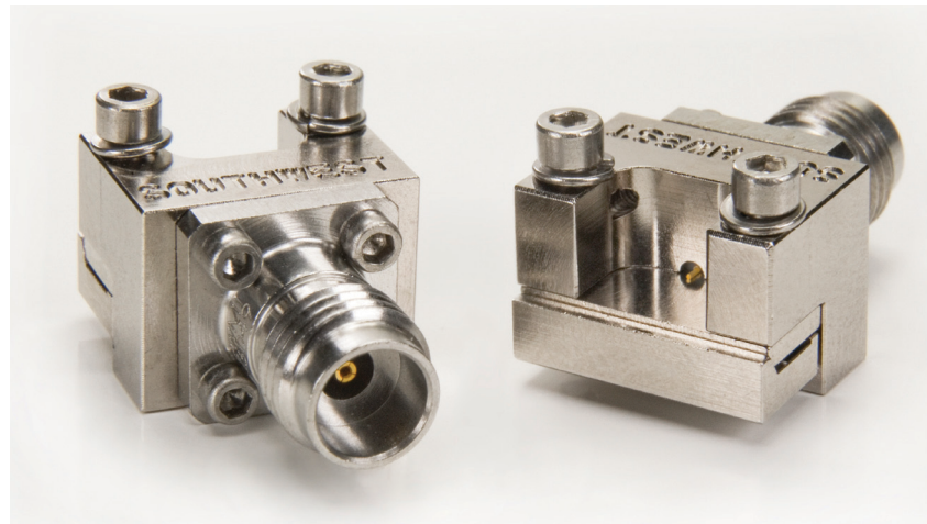
Front and back views of SMI 2.40 mm (50 GHz) End Launch Assemblies.
