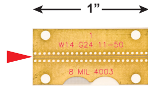
8 MIL R04003 GCPWG Test Board
