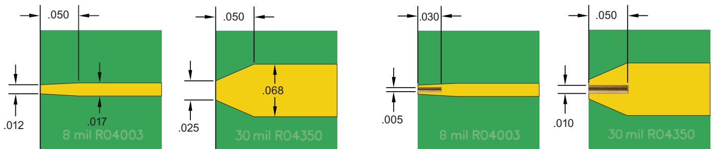
8 mil & 30 mil Straight Microstrip final board layout dimensions.
