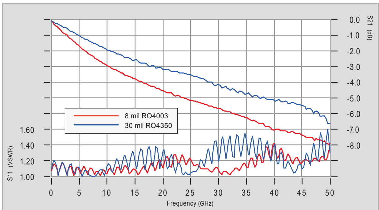
Actual Test Data for 2.5" GCPWG Test Boards.
