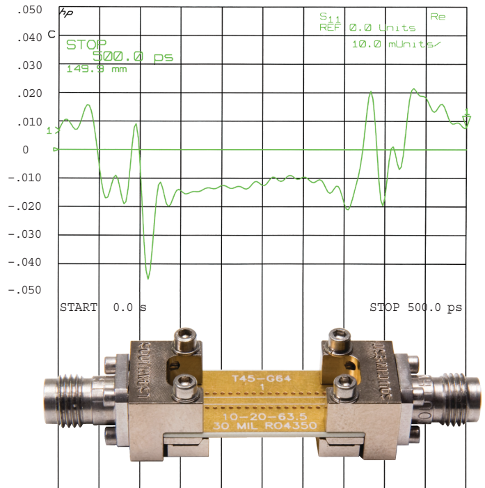
TDR of original coplanar test board (Serial Number 0).
