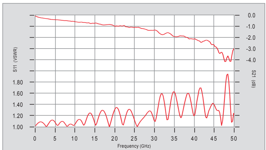
Test data original 30 mil GCPWG test board (Serial Number 0).
