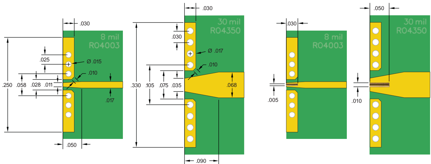
8 mil and 30 mil Top Ground Microstrip pin sizes relative to the board thickness.
