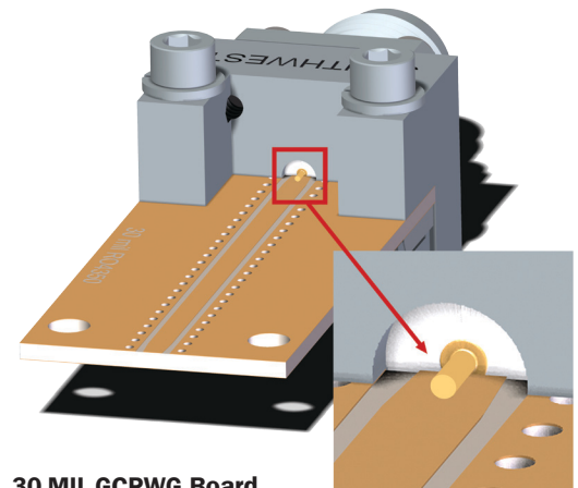
30 MIL GCPWG Board
