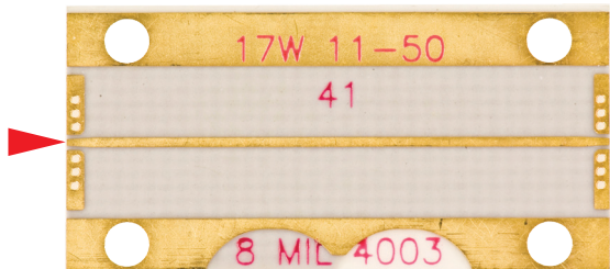
8 MIL R04003 Top Ground Microstrip
