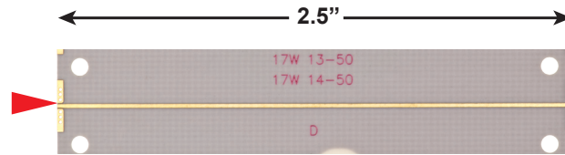
8 MIL RO4003 Top Ground Microstrip Test Board
